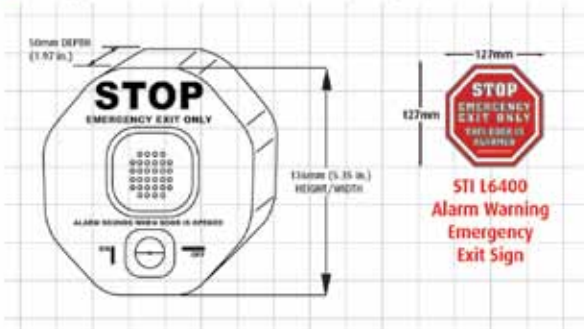
Exit Stopper dimensions and technical information (STI 6400)
